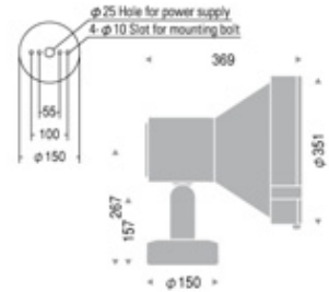
HIT 250W G12
